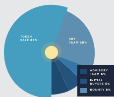
Token Distribution
